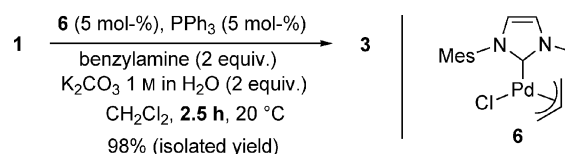
Scheme 2. Allylic amination using the well-defined [(\text{NHC})\text{Pd}(\text{allyl})\text{Cl}] complex 6 and \text{PPh}_3 under biphasic conditions.
