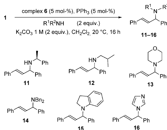
Scheme 7. Scope of the reaction: nitrogen nucleophiles.
