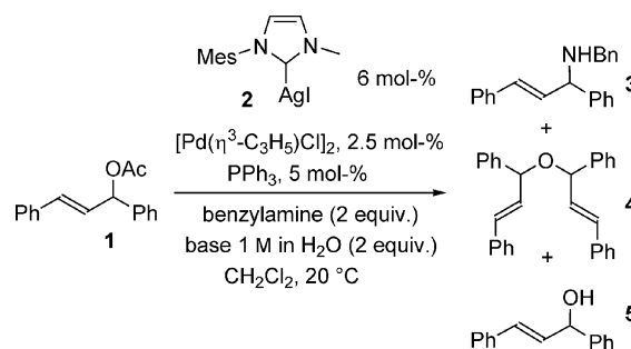
Scheme 1. Allylic amination using an [(\text{NHC})\text{Pd}(\text{allyl})\text{Cl}] complex generated in situ in the presence of \text{PPh}_3 .
