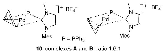
Figure 2. Coordination modes of the allyl ligand in complex 10 .
