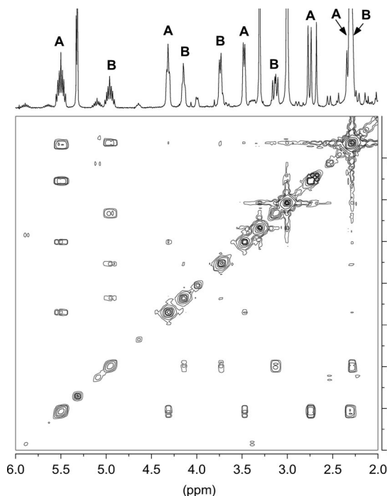
Figure 3. 2D ^1\text{H} -COSY spectrum of complex 10 at -15^\circ\text{C} .
