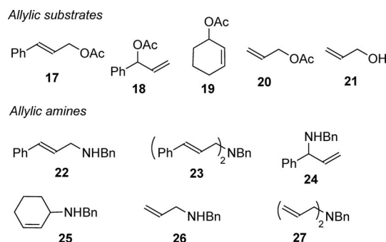
Figure 4. Allylic acetates, alcohol, and amines.
