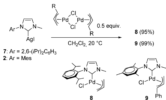
Scheme 4. Synthesis of well-defined [(NHC)Pd(allyl)Cl] complexes 8 and 9 .
