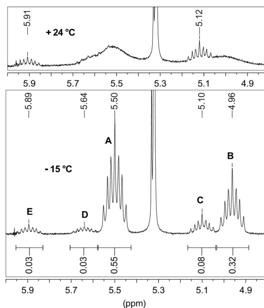
Figure 1. ^1\text{H} NMR spectra of complex 10 recorded at +24 and –15 °C (central allylic \text{CH} ).
